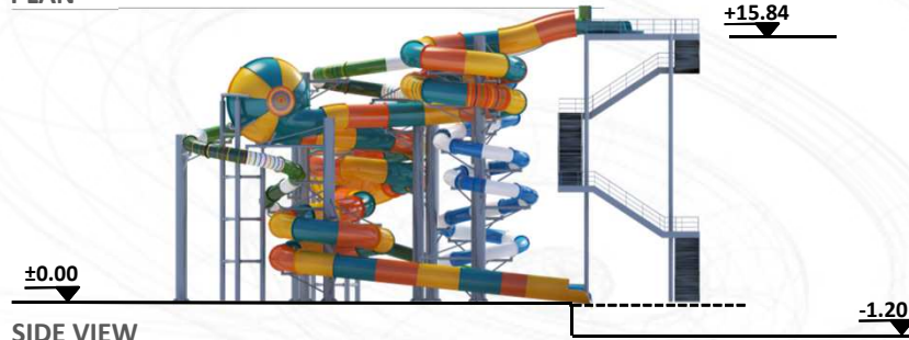
SIDE VIEW
